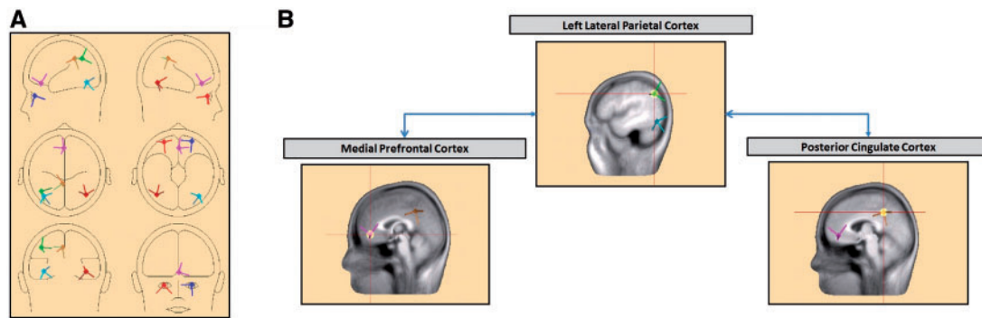
Fig. 1 Source model used for analyses. (A) The seven source model including eye and occipital sources. (B) Sources used to calculate phase-locking estimates within default mode network regions.
